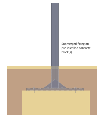
Submerged Fixing
