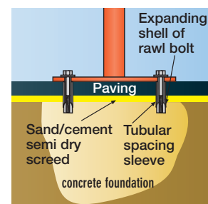
Surface fixed.
