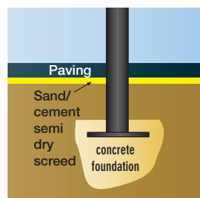
Submerged fixing.
