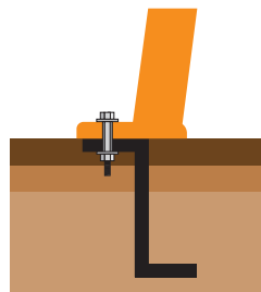
Extension Legs
