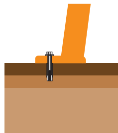
Ground Bolting
