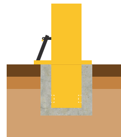
Removable Socket Fixing
