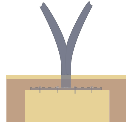
Submerged Fixing
